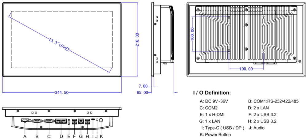
Panel Cutout Dimensions: 331 x 202 mm (13.03 x 7.95 in )
