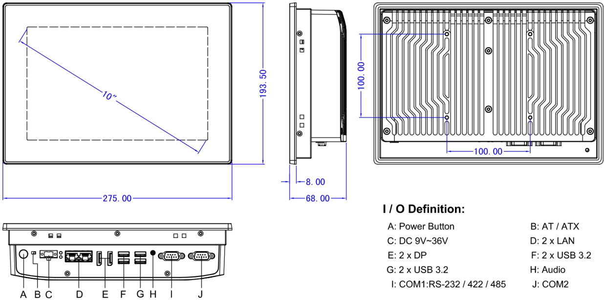
Panel Cutout Dimensions: 263 x 182 mm (10.35 x7.16 in )
