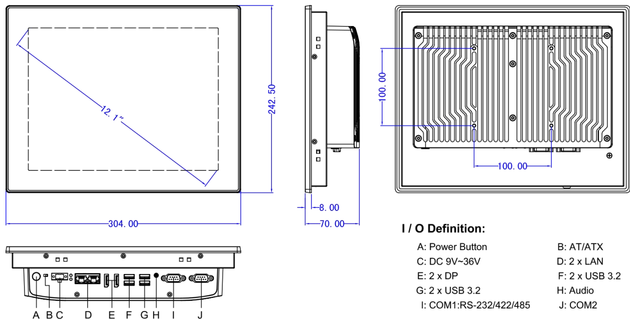
Panel Cutout Dimensions: 290 x 229 mm (11.42 x 9.0 in )
