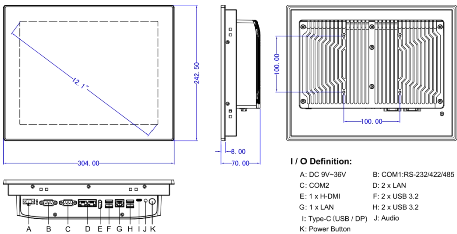
Panel Cutout Dimensions: 290 x 229 mm (11.42 x 9.0 in )
