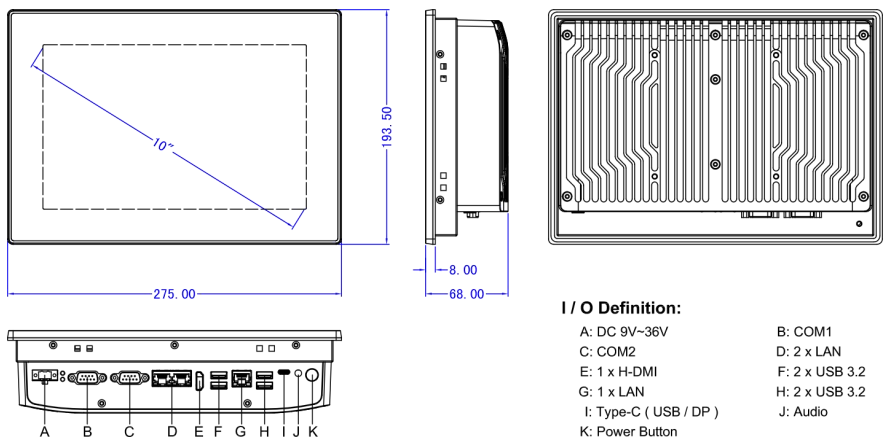
Panel Cutout Dimensions: 263 x 182 mm (10.35 x7.16 in )
