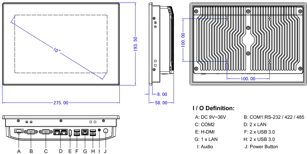
Panel Cutout Dimensions: 263 x 182 mm (10.35 x7.16 in )
