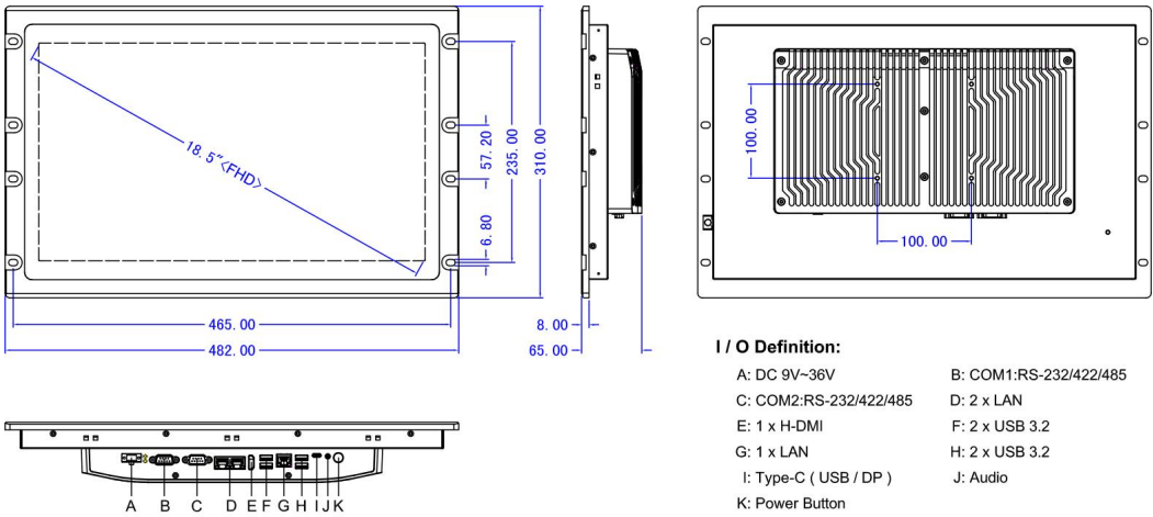
Panel Cutout Dimensions: 452 x 273 mm (17.80 x 10.75 in )
